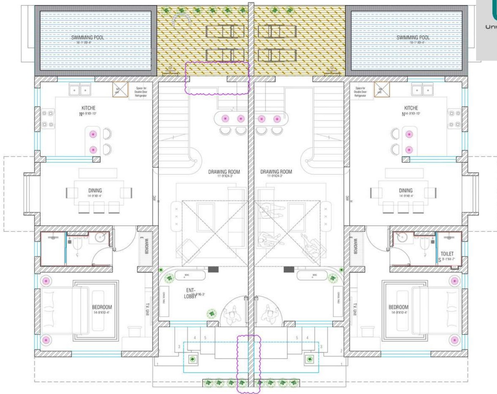
GROUND FLOOR LAYOUT PLAN
