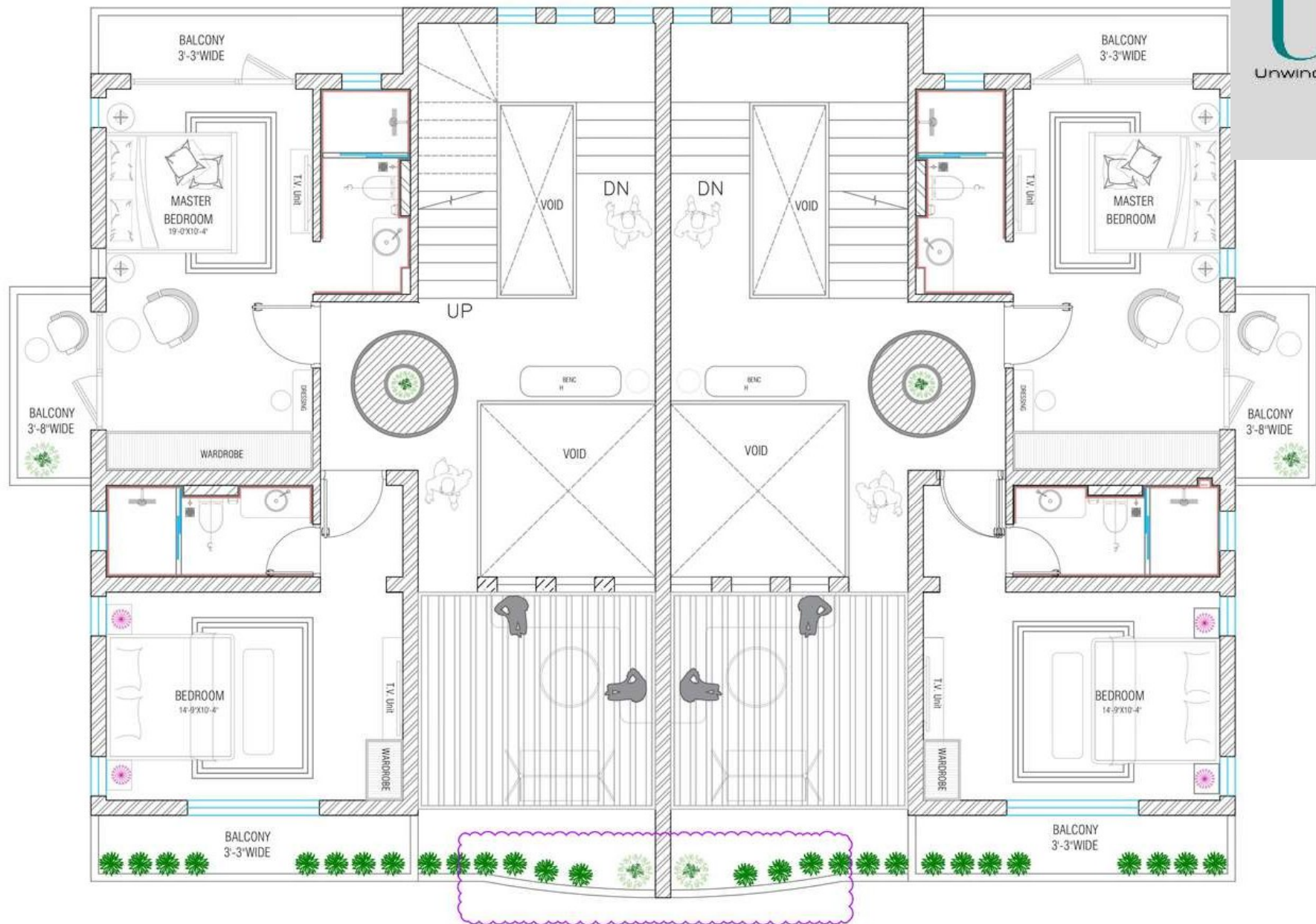
FIRST FLOOR LAYOUT PLAN
