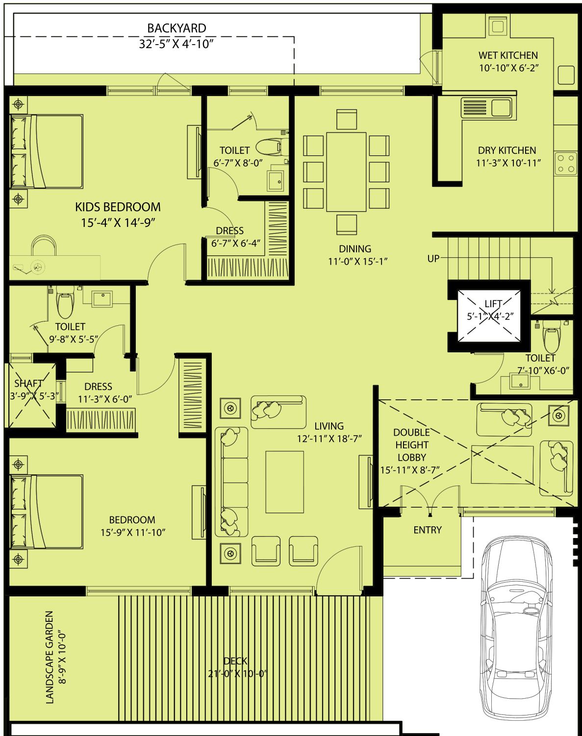
300 YARDS GROUND FLOOR PLAN
