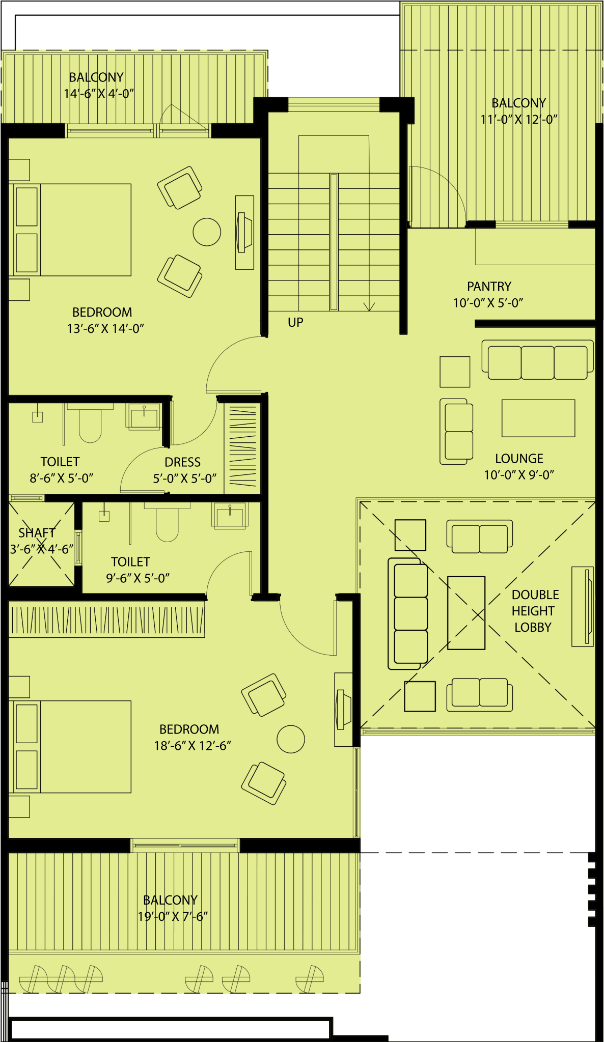
200 YARDS FIRST FLOOR PLAN
