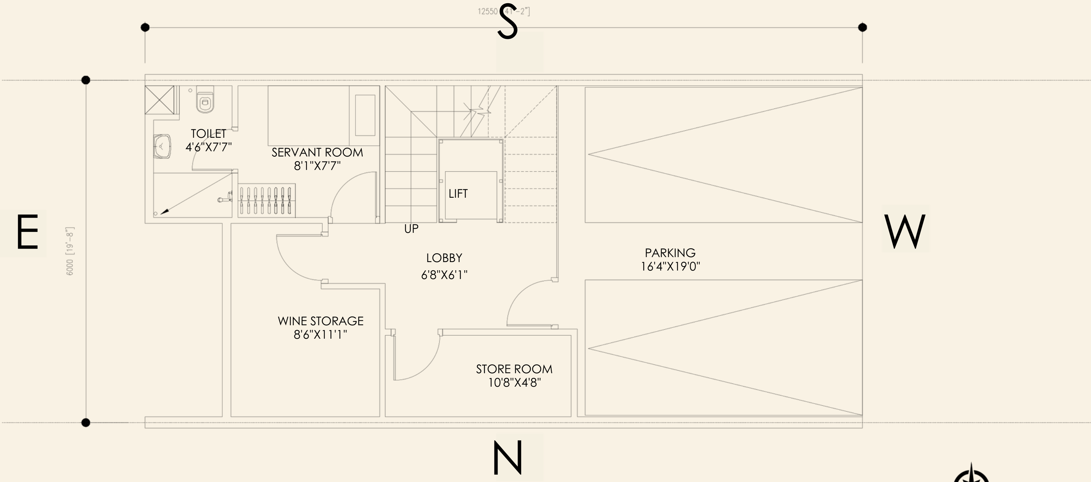
BASEMENT PLAN
